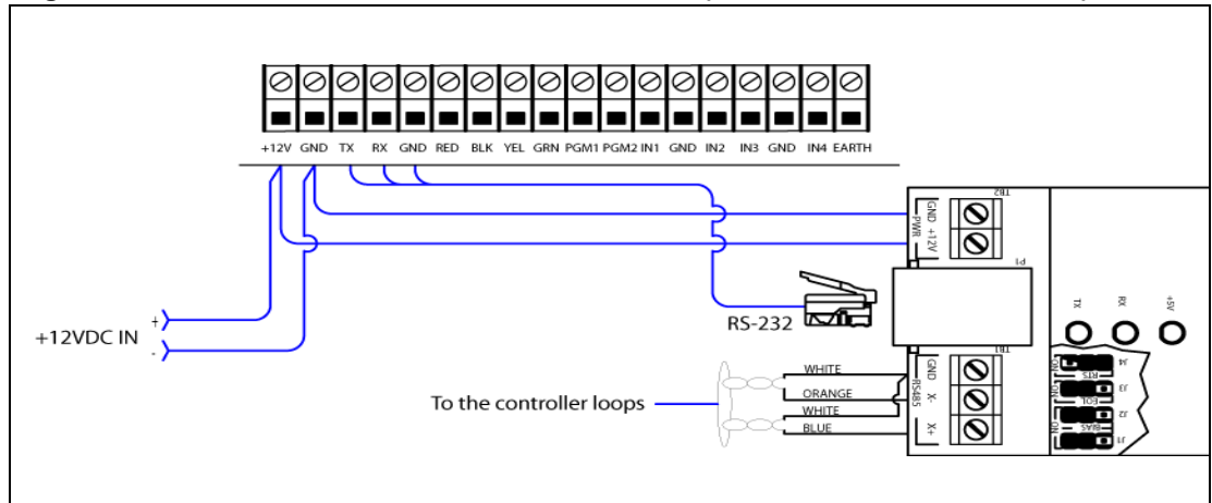
Figure 1: RS-232 connection with RJ12 to VC-485 (KT-100, KT-200 and KT-300)
