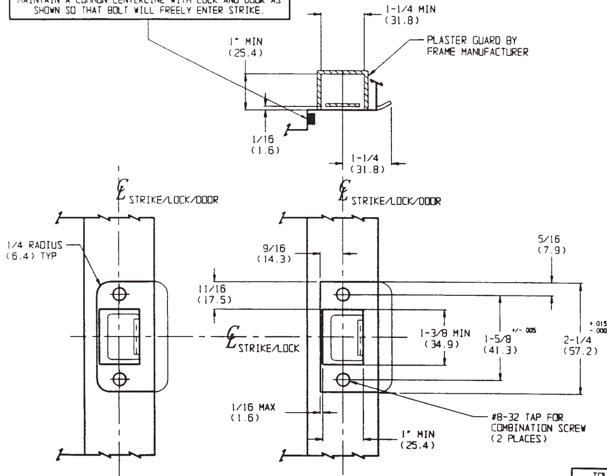
FRAME DETAIL WITH ROUNDED CORNERS
