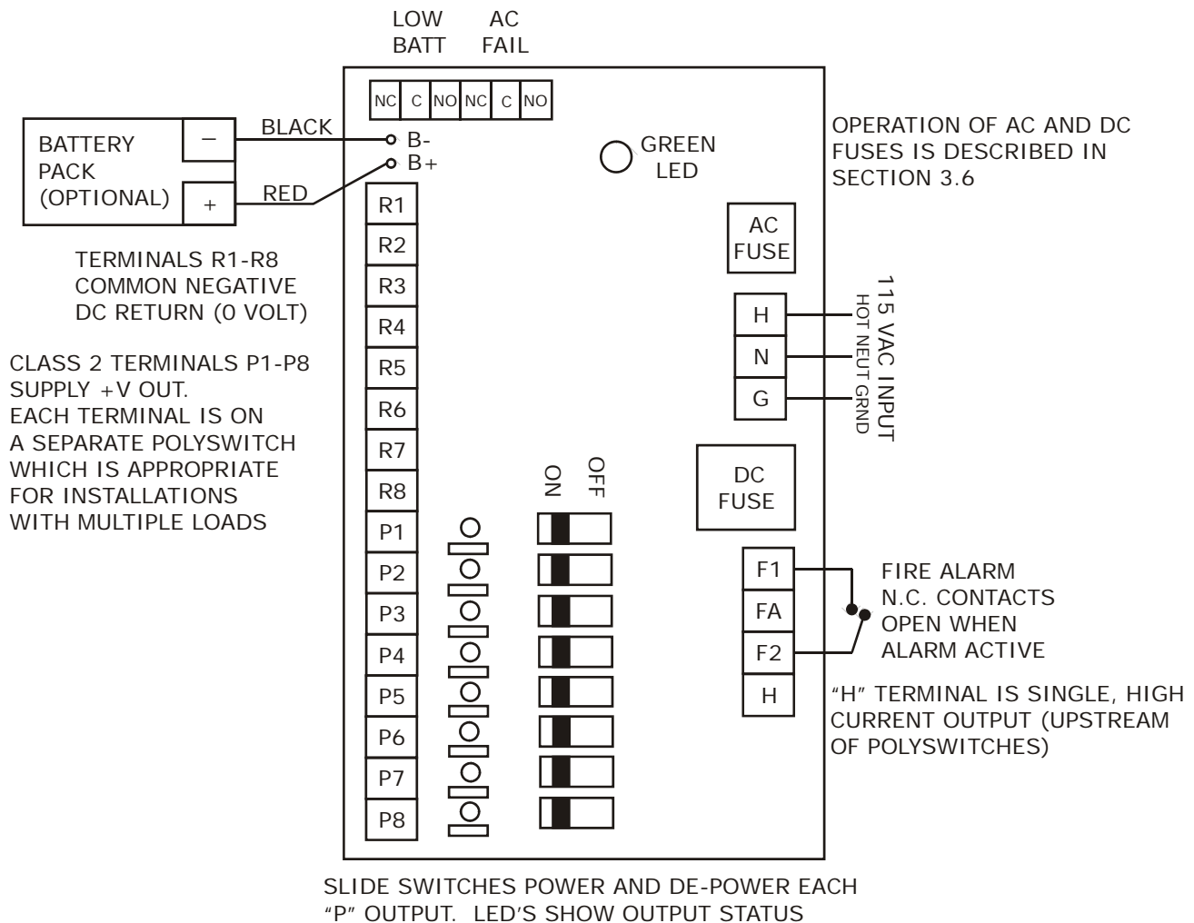
FIG. 1: POWER SUPPLY WIRING WITH CCS8M BOARD
