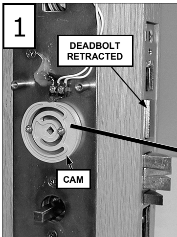
FIG. 1: CAM OVERVIEW.
