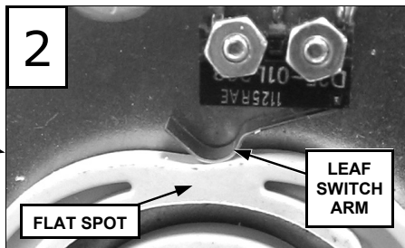
FIG. 2: CLOSE-UP OF CAM FLAT SPOT.
