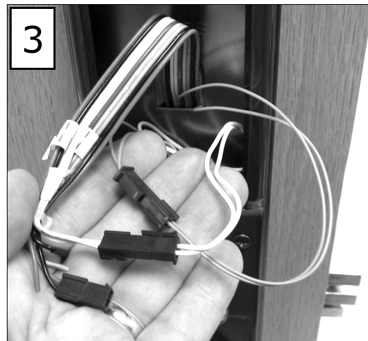
FIG. 3: CONNECT PLUGS.
